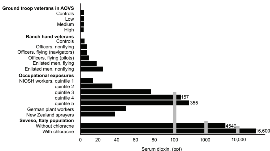
FIGURE 2-2 Median serum TCDD levels in various study populations.
